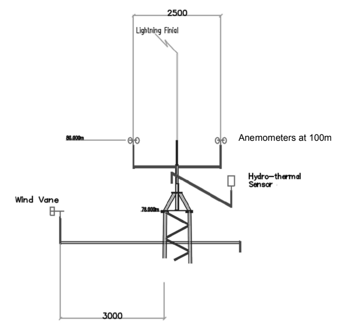
Tower Peak, Sliding Pole and Typical Booms
