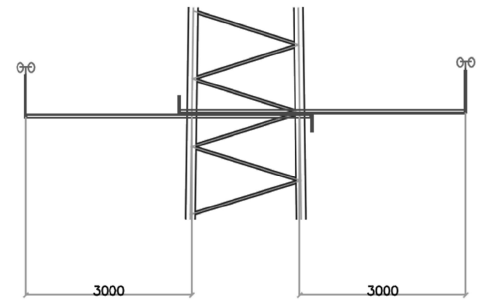
Typical Anemometer Support Booms
