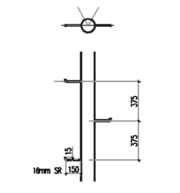
Climbing Step Bolts on one leg
